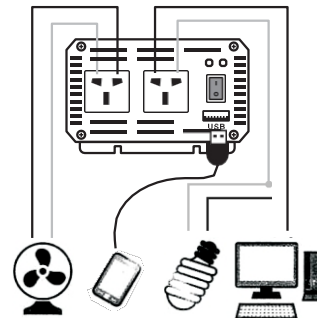
Outputs connection
