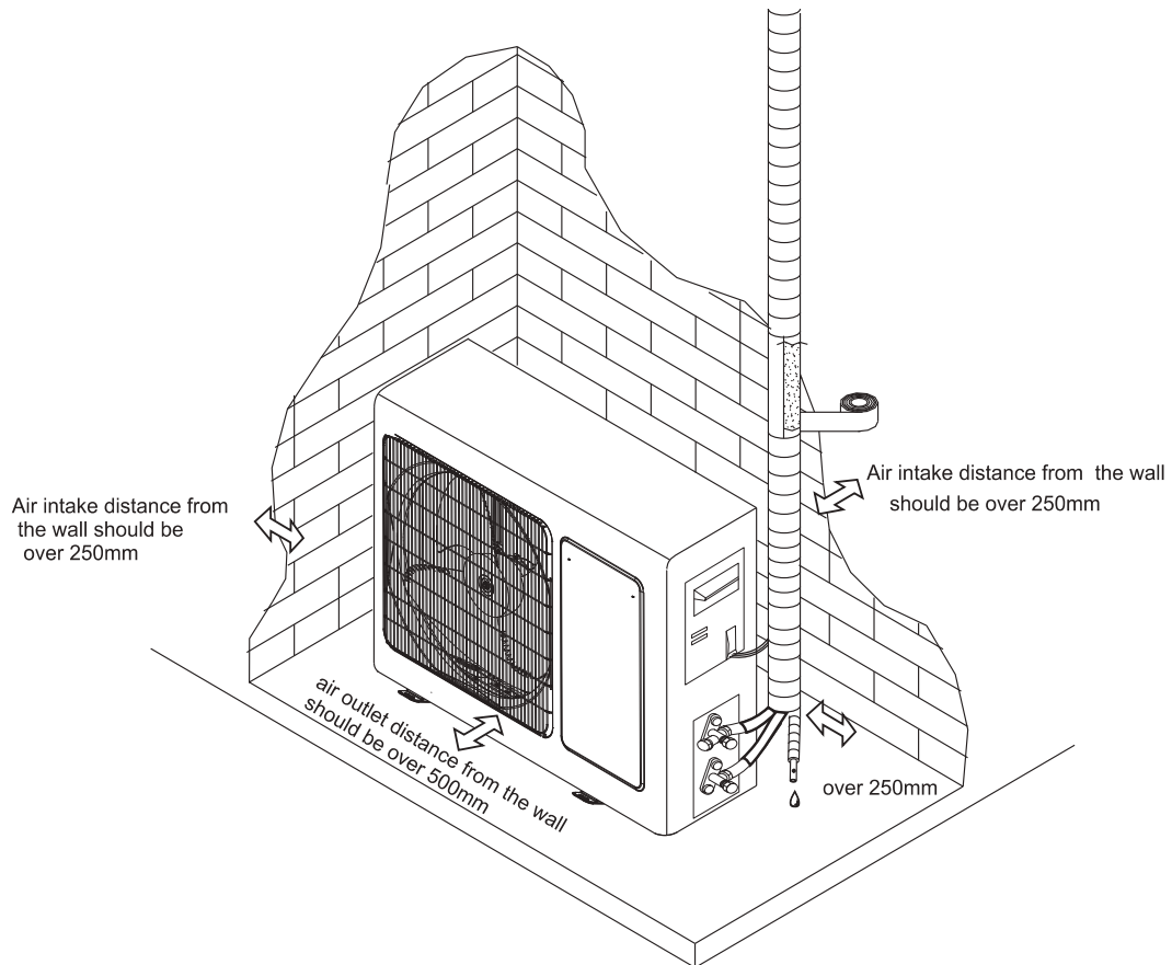
outdoor unit
