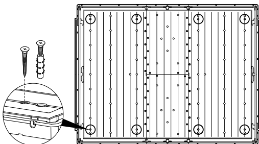
NEWTON PLUS 975 WIDE OPTION
