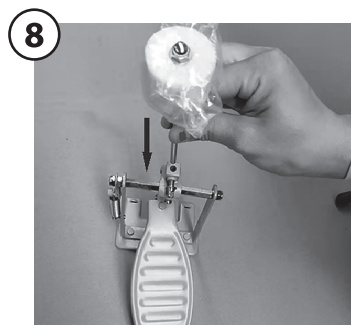
8 Insert the Beater. Into the top hole of the pedal as shown in the image and adjust it.
