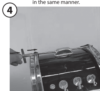
4 Use 4 short straight metal bars. Attach them around the drum as shown in the image.
