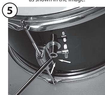
5 Use two short metal bars. Fix the drum and insert them into the holes, as shown in the image.
