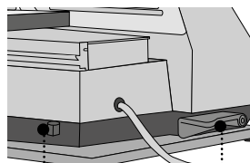
Release button Swivelling lever
