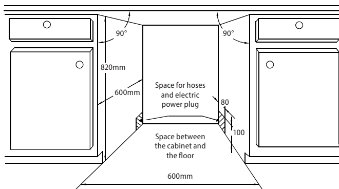
Dishwasher Open the appliance door. Lower cabinets Minimum space: 50 mm
